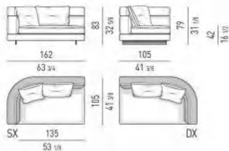
ELEMENTO TERMINALE HIGH CM 162 ELEMENT WITH ONE ARMREST HIGH CM 162
