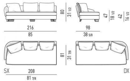
LARGE ELEMENT WITH 1 ARMREST CM 216
