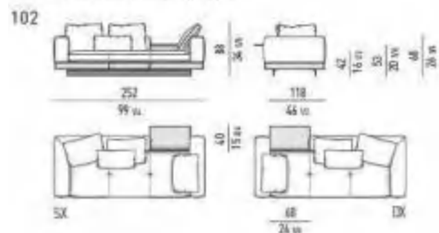
DIVANO-DAYBED CON FLAP CM 252 DAYBED-SOFA WITH FLAP CM 252
