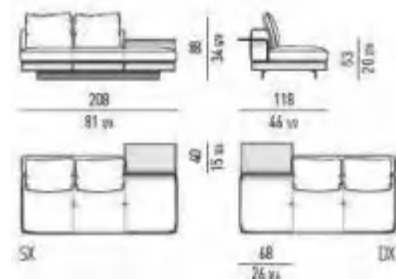
ELEMENTO PENISOLA CON FLAP CM 208 OPEN-END ELEMENT WITH FLAP CM 208
