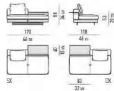
ELEMENTO PENISOLA CON FLAP CM 170 OPEN-END ELEMENT WITH FLAP CM 170
