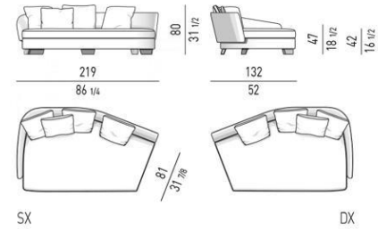
LARGE SOFA CHAISE-LONGUE
