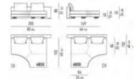
OFFSET SOFA CHAISE-LONGUE CM 205X169 - SEAT CM 86
