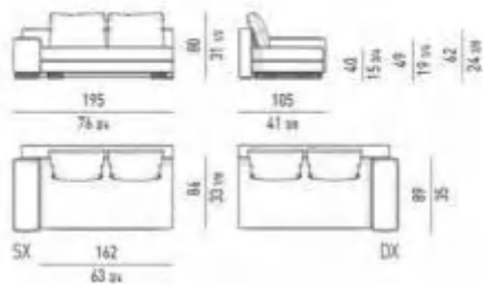
ELEMENT WITH ONE ARMREST CM 195
