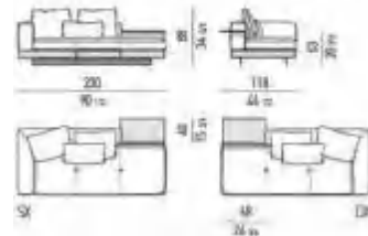
ELEMENTO TERMINALE PENISOLA CON FLAP CM 230 OPEN-END ELEMENT WITH 1 ARMREST AND FLAP CM 230
