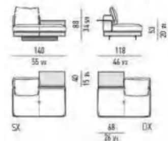
ELEMENTO PENISOLA CON FLAP CM 140 OPEN-END ELEMENT WITH FLAP CM 140
