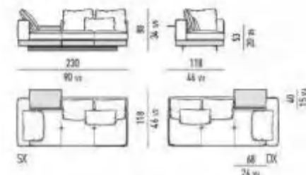
ELEMENTO DAYBED CON FLAP CM 230 DAYBED ELEMENT WITH FLAP CM 230
