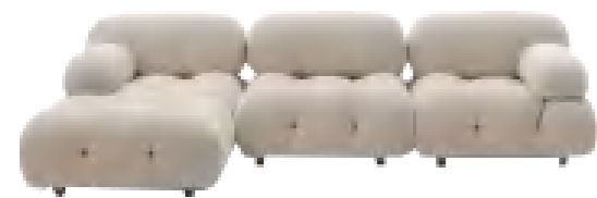
魔方沙发 座950*950*400mm 脚踏950*620*400mm 扶手620*310*340mm 背950*310*300mm
