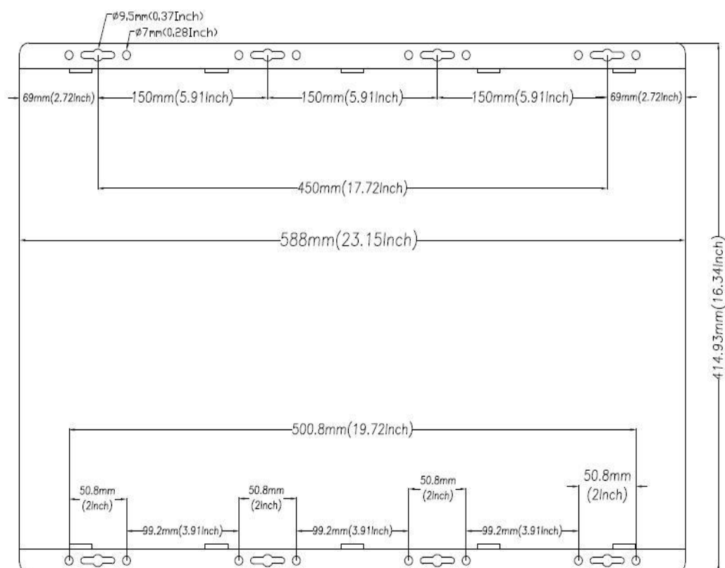
HP8-12KW Model HPV8-12KW Model
