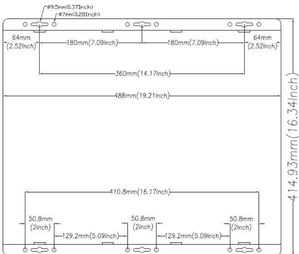
HP4-6KW Model HPV1-6KW Model
