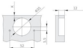
孔距:52mm
