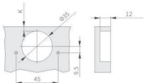
孔距:45mm
