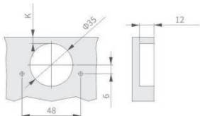
孔距:48mm
