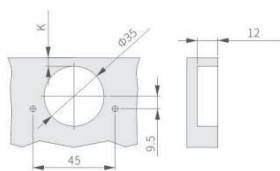
孔距:45mm
