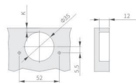
孔距:52mm
