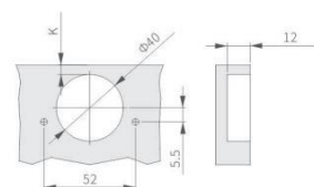
孔距:52mm
