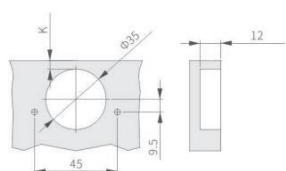
孔距:45mm
