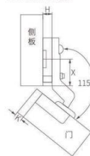
30° hinges 30°铝框铰链
