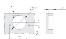
孔距:52mm
