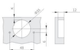
孔距:48mm
