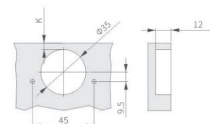
孔距:45mm
