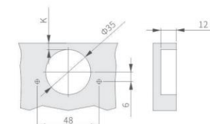
孔距:48mm
