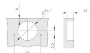
孔距:52mm
