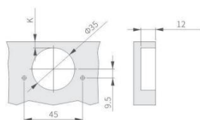
孔距:45mm
