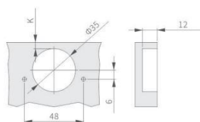
孔距:48mm
