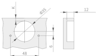
孔距:48mm
