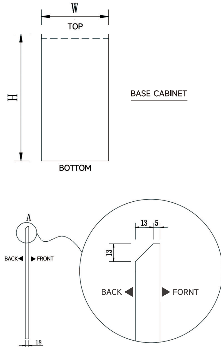
DETAILED DRAWING OF LOCATON A
