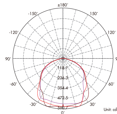
Lux distance Curve (3000K, 110°) .....
