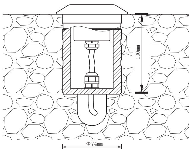
Marine RC recessed with mounting box
