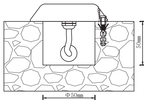
Marine SF surface mounted with screws
