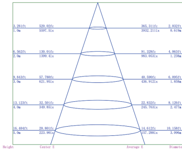
Lux distance Curve (3000K, 36° )
