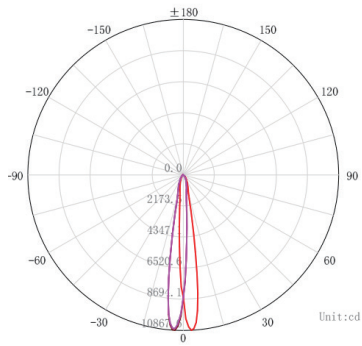
Lux distance Curve (3000K, 15° )
