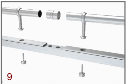
Handrail
