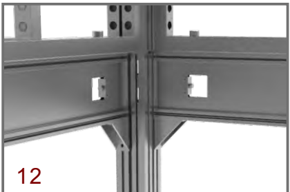
90° Reinforcement parts
