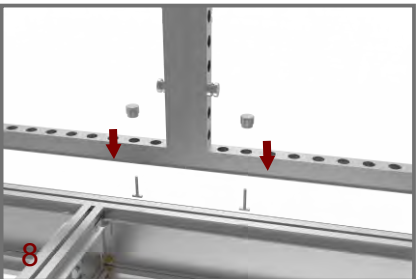
Frames connection
