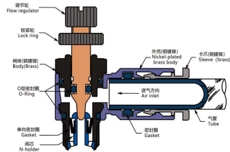
进气节流阀 /Air inlet controller
