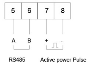
10(60)A specification wiring diagram
