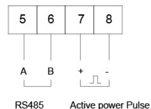
20(100)A specification wiring diagram
