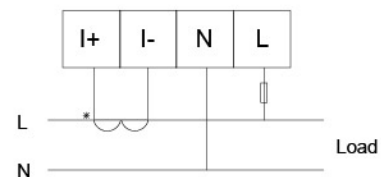
10(60)A specification wiring diagram
