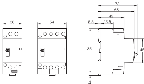
BCH8 Manual Contactor 32/40/63A
